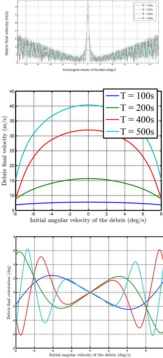
Figure 4. Debris final velocity and orientation as a function of initial residual spin.
