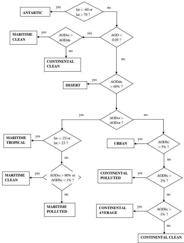
Fig. 1. Sketch of the algorithm converting the total optical depth (AOD) and partial optical depths of MACC species – dust (AODdu), sea salt (AODss), black carbon (AODbc), and organic matter (AODor) – into aerosol types: urban, continental clean, continental polluted, continental average, maritime clean, maritime polluted, maritime tropical, Antarctic, and desert. “lat” is latitude.
