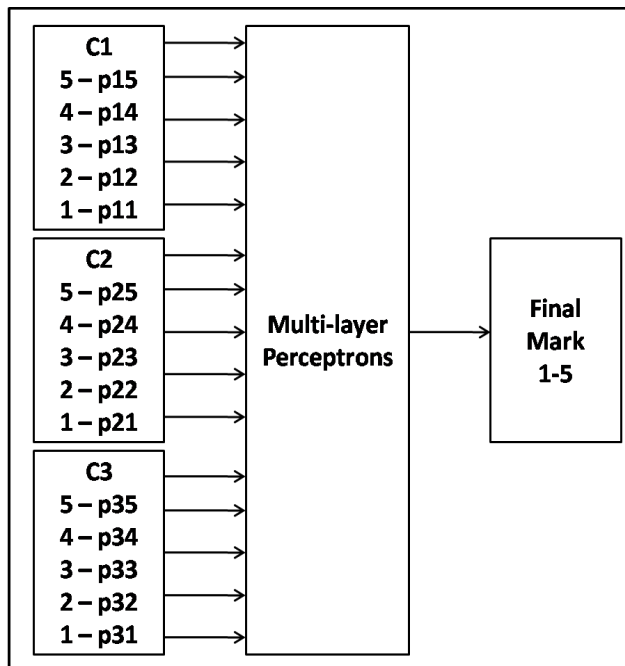
Figure 5. Multi-Layer Perceptrons
