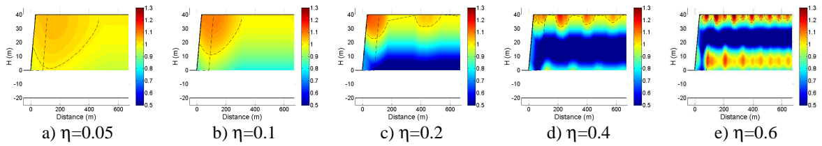
Figure 10. Spatial distribution of the horizontal acceleration amplification for slopes with the same value of slope height ( H=40\text{m} ), the same slope angle ( \alpha=50^\circ ) but different values of dimensionless frequency
