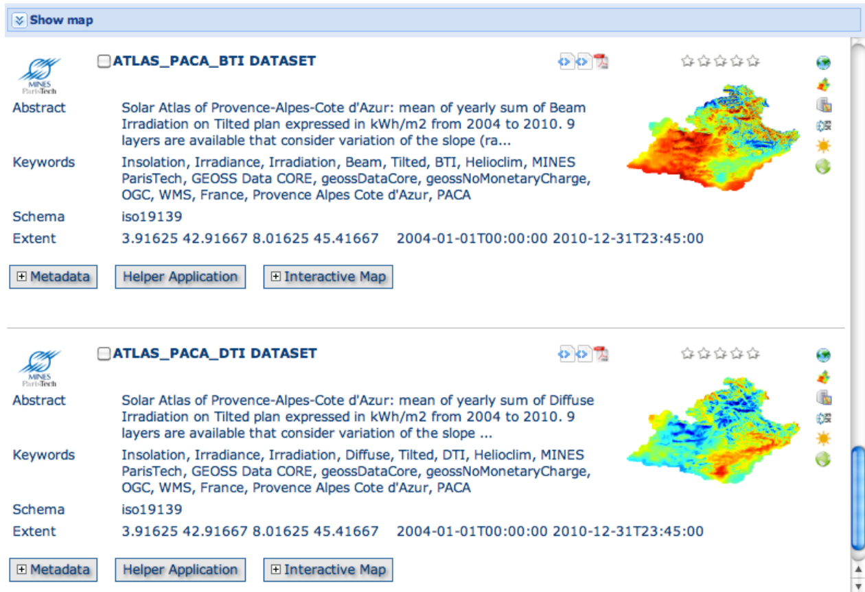
Figure 9: Implementation of Helper Application as an ISO 19139 Metadata Tag
