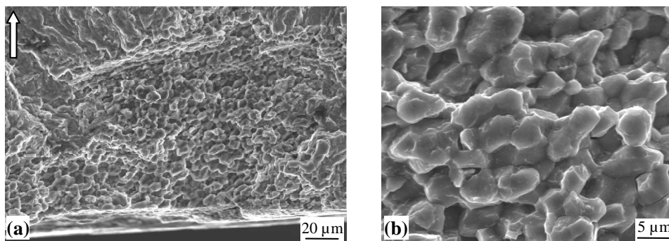
Figure 8. (a) Fatigue crack initiation from "sensitive" GBs of a Gap3 bearing specimen, \Delta\sigma = 256 \text{ MPa} , lifetime \sim 26,500 cycles. The average crack propagation is indicated with a white arrow and the specimen orientation is the same as in Fig. 7a. (b) Detailed view of intergranular fracture of "sensitive" GBs
