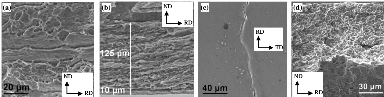
Figure 4. (a,b,d) fracture surfaces (a) in the TMAZ (sound and JLR bearing welds), (b) of a KB bearing weld (the striated zone corresponding to the KB defect itself) and (d) close to the root of a Gap7 weld. (c) Onset of cracking at the lower surface of a KB bearing specimen, slightly polished and then pulled in tension in the SEM (loading axis horizontal)
