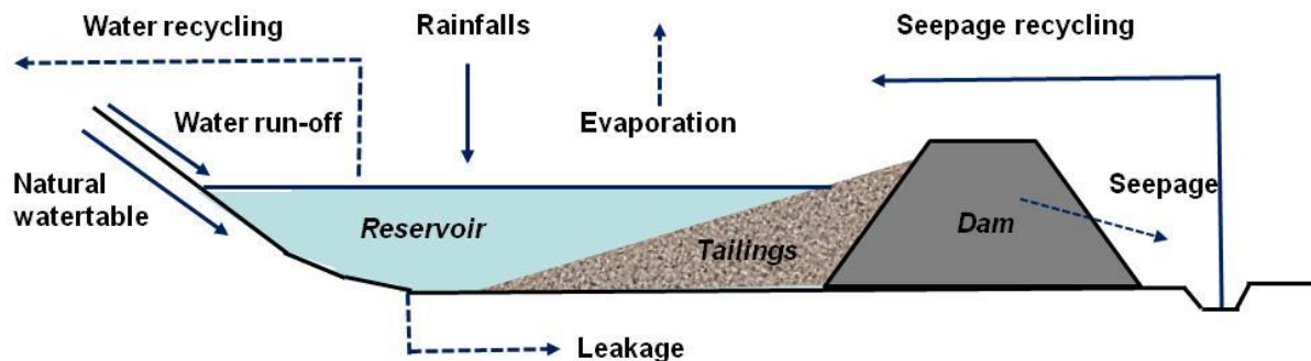
Figure 17: Schematic hydraulic assessment
