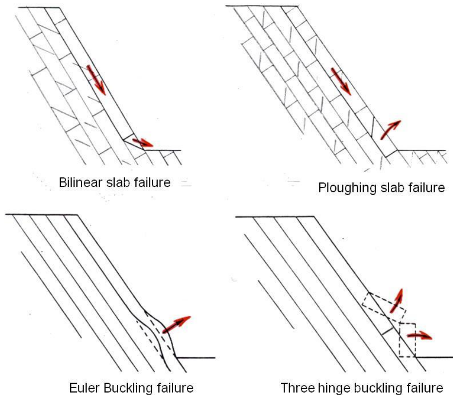
Figure 4 : Footwall elementary slab failure mechanisms (after P.M. Hawley, 1985)
