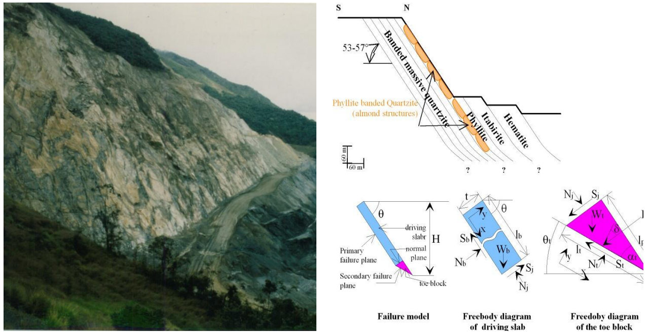
Figure 9 : South slope face of the Timbopeba mine in Brazil: bilinear slab potential failure mechanism
