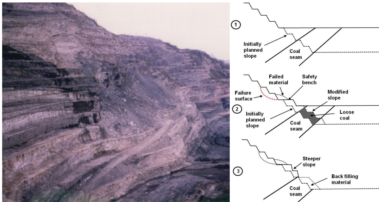
Figure 6 : West slope face of Decazeville coal mine: general view and slope instability (left) and slope management (right)
