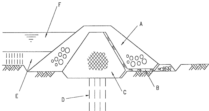
(A) Shoulder fill; (B) Filter drainage system; (C) Core; (D) Foundation grouting; (E) Deposited tailings; (F) Water in reservoir
