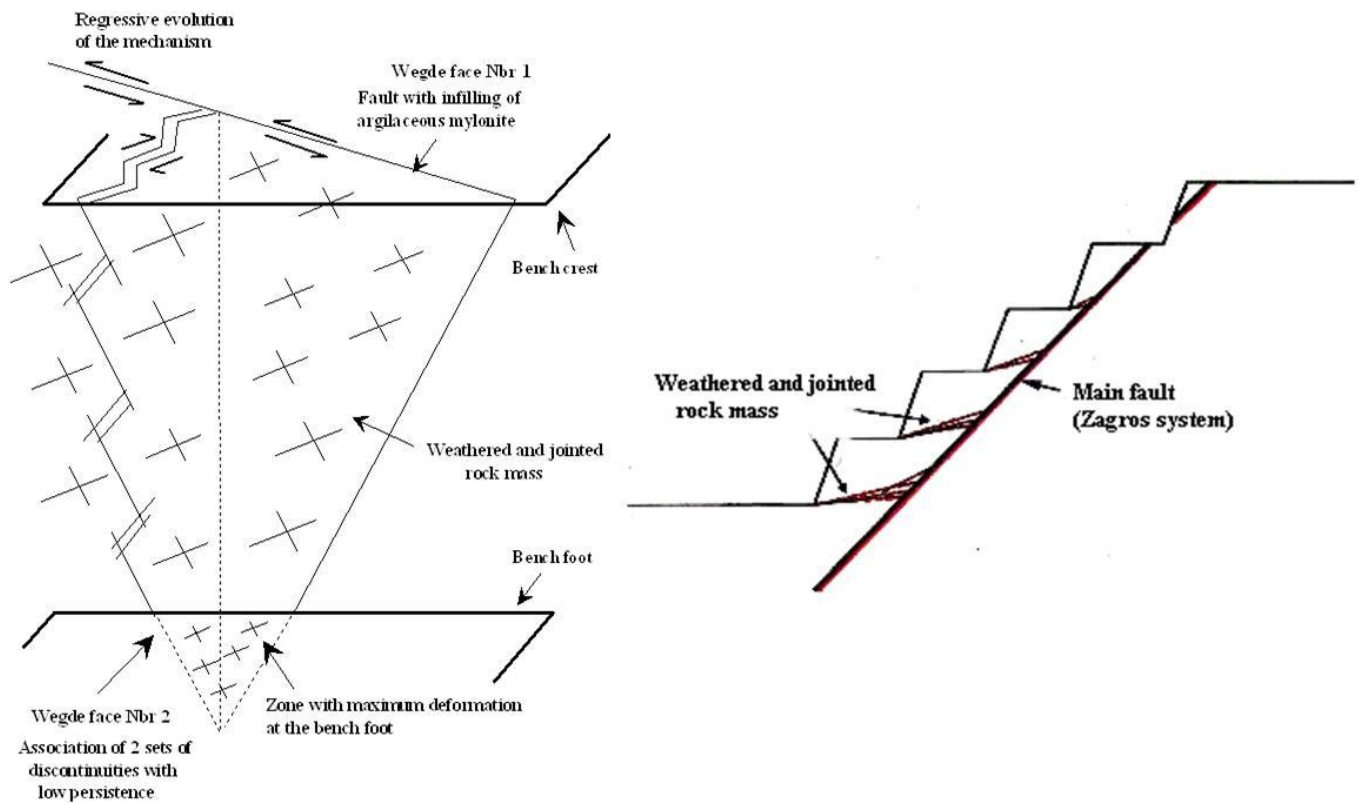
Figure 8 : Plane or wedge failure mechanism cinematically possible only if the rock material (highly weathered and jointed) can fail.
