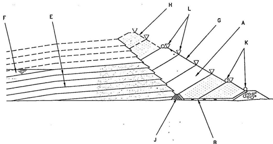
(A) Structural zone formed with hydrocyclone underflow; (B) Filter drain; (E) Beach formed with hydrocyclone overflow; (F) Water in reservoir; (G) Current embankment profile; (H) Future embankment profile; (J) Starter dam; (K) Successive tailings pipeline locations; (L) Successive hydrocyclone or deposition locations
