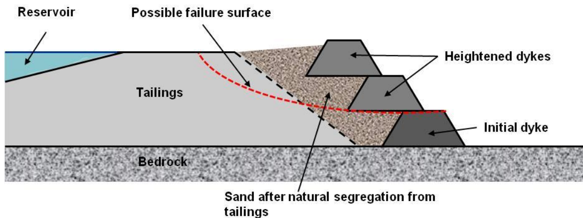
Figure 14: Possible surface failure location in upstream constructed tailing dam
