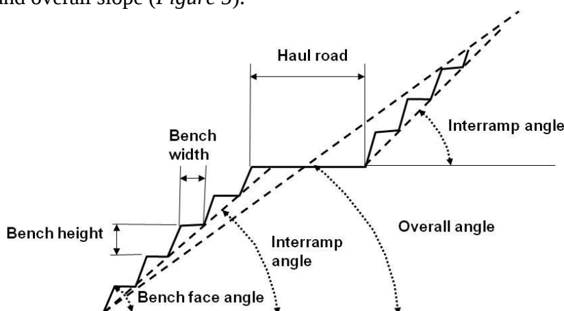
Figure 5: Typical slope design cross section
