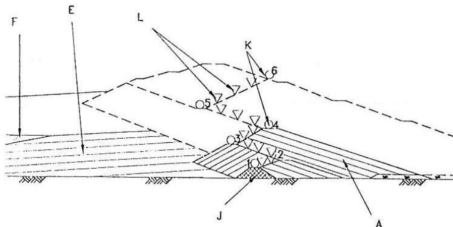
(A) Structural zone formed with hydrocyclone underflow; (B) Filter drain; (E) Beach formed with hydrocyclone overflow; (F) Water in reservoir; (G) Current embankment profile; (H) Future embankment profile; (J) Starter dam; (K) Successive tailings pipeline locations; (L) Successive hydrocyclone or deposition locations
