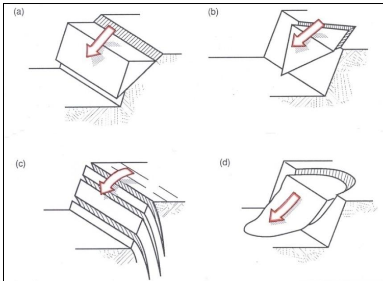
Figure 3: Some elementary processes of slope failure: (a) plane failure, (b) wedge failure, (c) toppling failure, (d) circular failure (modified after Hoek and Bray, 1981)
