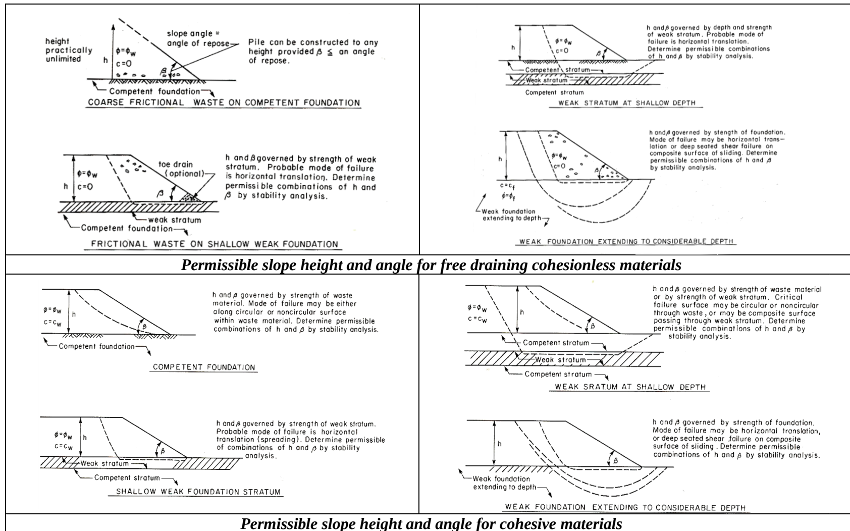
Figure 10: Permissible slope height and angle of waste dump (after CANMET, 1977)
