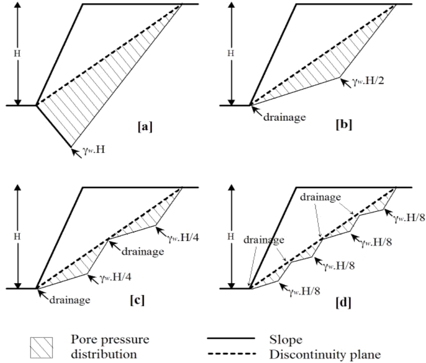
Figure 2 : Schematic possible drainage conditions and pore pressure distribution along the discontinuity plane
