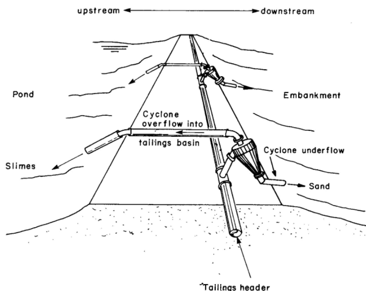
Figure 11: Typical hydrocycloning arrangement (after ICOLD, 1996)
