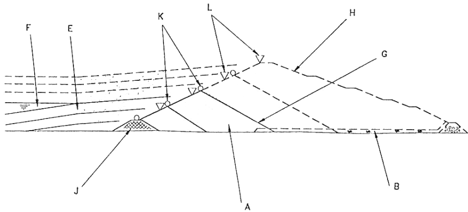
(A) Structural zone formed with hydrocyclone underflow; (B) Filter drain; (E) Beach formed with hydrocyclone overflow; (F) Water in reservoir; (G) Current embankment profile; (H) Future embankment profile; (J) Starter dam; (K) Successive tailings pipeline locations; (L) Successive hydrocyclone or deposition locations.
