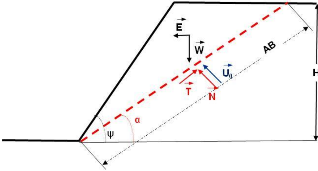
Figure 1: Equilibrium of a block sliding on a plane failure surface
