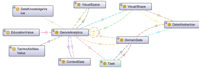
Fig. 2. Geovisual analytics model onotlogy in Protégé
