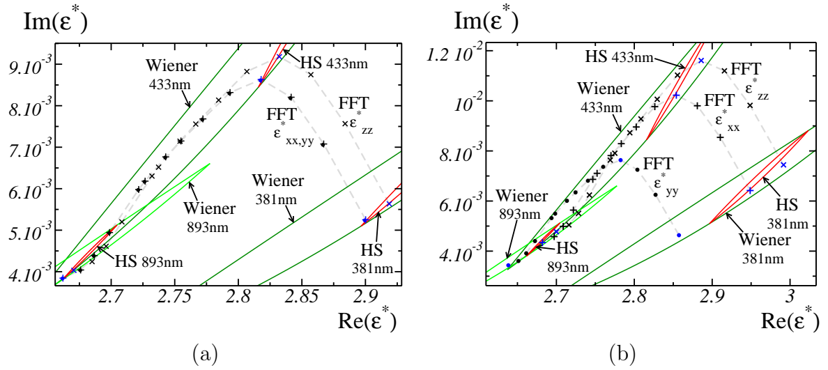
Figure 6: Cole-cole plots of the effective permittivity components \epsilon_{xx,yy,zz}^* (symbols +, • and \times resp., joined by dotted gray lines), as computed by FFT, for a deposit microstructure made of spheres (a) or aligned rhombi inclusions (b) with volume fraction 18%. The wavelength takes the values \lambda = 381, 400, 416, 433, 455, 480, 505, 527, 562, 575, 650, 706, 771, and 893\text{nm} (right to left). Domains delimited by the Wiener and Hashin-Shtrikman's bounds are shown in green and red, resp., for the values \omega = 381, 893 and 433\text{nm} with corresponding FFT results shown in blue.
