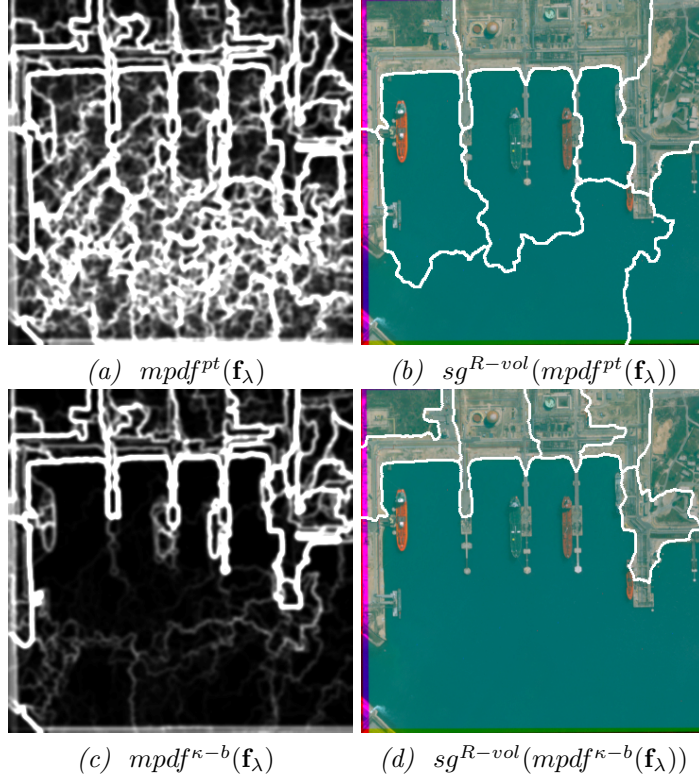
Figure 11. Comparison between (a) the pdf mpdf^{pt}(\mathbf{f}_\lambda) and (b) the associated stochastic WS with uniform random point germs with a volume criterion sg^{R-vol}(mpdf^{pt}(\mathbf{f}_\lambda)) to (c) the pdf mpdf^{\kappa-b}(\mathbf{f}_\lambda) and (d) the associated stochastic WS with regionalized random ball germs with a volume criterion sg^{R-vol}(mpdf^{\kappa-b}(\mathbf{f}_\lambda)) . Only R = 8 regions with the largest volume are retained. For visualization, the contours of the segmentations are dilated by a SE of size 3 \times 3 pixels.
