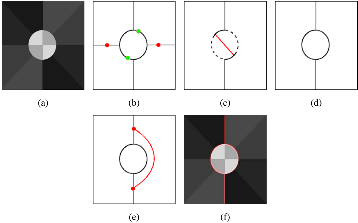
Fig. 62: (a) Initial image, (b) segmentation level s_1 with, in red, the minima of h_1 and, in green, two FOZ on the boundary of the central catchment basin. (c) Result of the watershed of h_2 , in red a watershed line marking the central CB as a WSZ (d). (e) and (f), final result, the ground is segmented.
