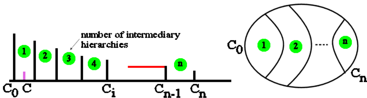
Fig. 40: Building a configuration where the oscillation period of contour C (purple contour on the left) is equal to n . The circled values correspond to the number of intermediary hierarchies inside the various catchment basins. In red, value of the hierarchical image at step n-1 . On the right, 2D representation of this configuration.
