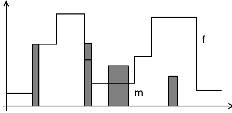
Fig. 9: Initial profile and marker function m . This function marks the cells which will be rebuilt and gives their new values.
