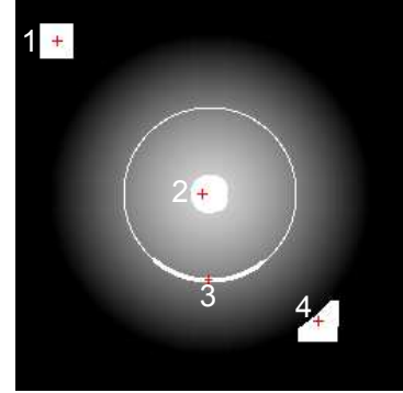
Figure 1. Four region growing structuring elements with N = 506 pixels. The central pixels of each SE (the seeds), are referenced by the crosses.
