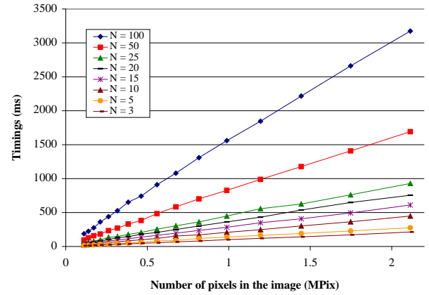
Figure 8. Linear w.r.t. n : Computation time of an erosion with REGSEs as function of the number of pixels in the image and for different size of SEs. This benchmark was made on a computer Intel Core (i7-870) CPU @2.93GHz using a multithreaded C++ implementation. (Images: Lena of increasing size)
