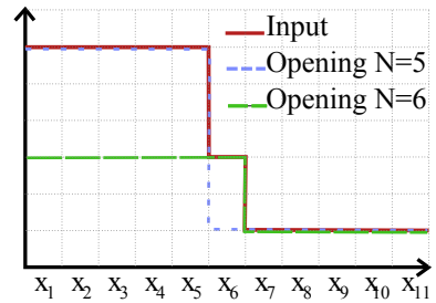
Figure 4. 1D signal and its corresponding REGSE openings of size 5 and 6 pixels.
