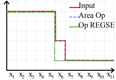
Figure 2. 1D signal and its corresponding area opening and REGSE opening. Size 3 pixels.
