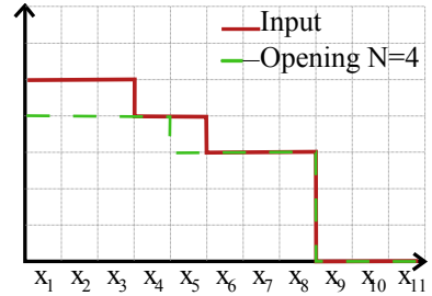
Figure 3. 1D signal and its corresponding REGSE opening of size 4 pixels.
