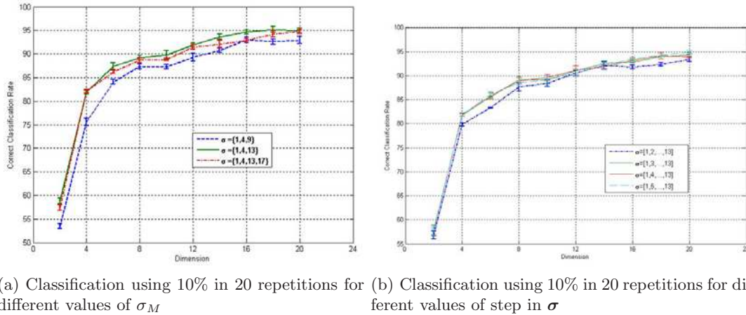
Figure 8. Indian Pine Classification using SVM for different scale parameters \sigma
