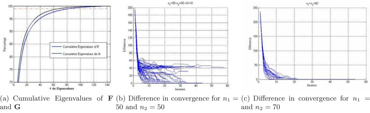
Figure 7. Comparison in convergence between two parameters sets in HOSVD tensor decomposition in Indian Pine HSI. The dimension utilized for HOSVD in the experiments is associated with the 99% of cumulate variance, in this case n_1 = 65 and n_2 = 82 .
