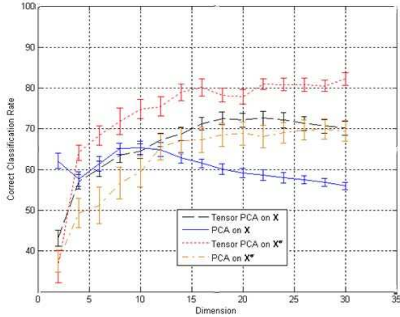
(b) 20 training samples in 9 classes in 20 random repetitions.
