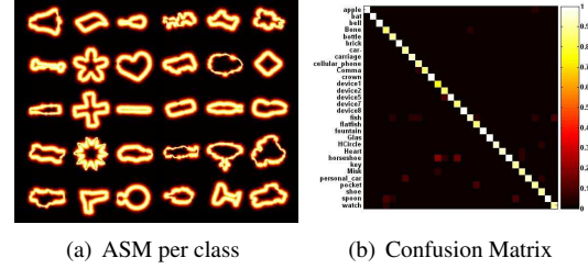
Figure 5. Associated probability map and confusion matrix for MPEG-7
