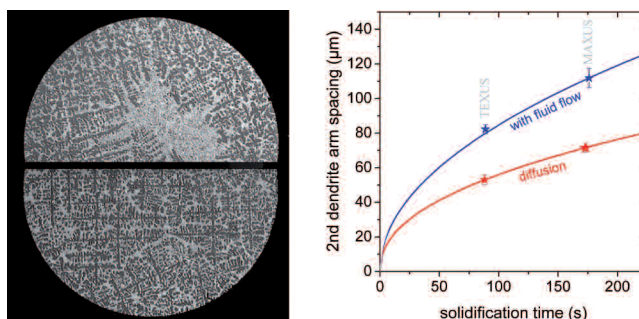
▲ FIG. 2: Solidification of Al 6wt%Si alloys in microgravity.
