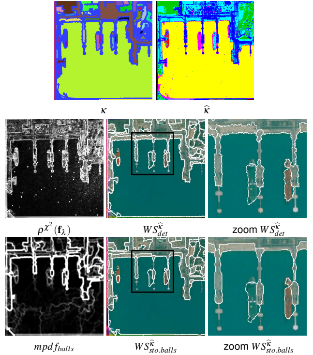
Figure 9. Filtered classification \hat{\kappa} , deterministic approach WS_{det}^{\hat{\kappa}} on Chi-squared metric based gradient \rho^{\chi^2}(\mathbf{f}_\lambda) (top) and stochastic approach WS_{sto.ball}^{\hat{\kappa}} on mpdf_{balls} (bottom) on image "Port de Bouc". In both cases, the seeds come from \hat{\kappa} . For visualization, and for complete segmented images the contours are dilated by a se of size 3 \times 3 pixels.
