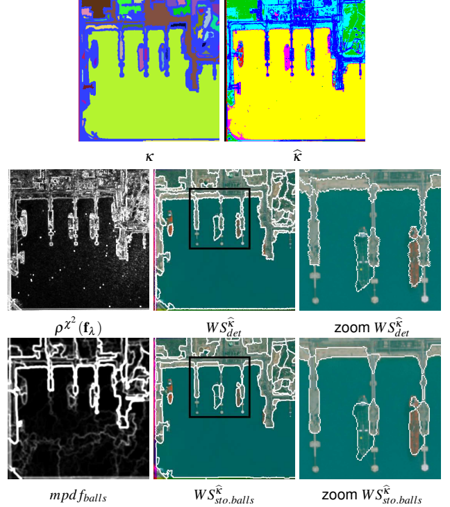
Figure 9. Filtered classification \hat{\kappa} , deterministic approach WS_{det}^{\hat{\kappa}} on Chi-squared metric based gradient \rho\chi^2(\mathbf{f}_\lambda) (top) and stochastic approach WS_{sto.balls}^{\hat{\kappa}} on mpdf_{balls} (bottom) on image "Port de Bouc". In both cases, the seeds come from \hat{\kappa} . For visualization, and for complete segmented images the contours are dilated by a se of size 3 \times 3 pixels.
