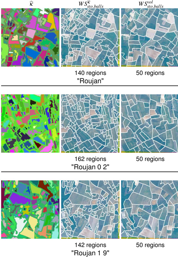
Figure 8. Comparison between segmentations of mpdf_{balls} by stochastic WS with a prior given number of regions R = 50 ( WS_{sto.balls}^{vol} ) or with seeds coming from the filtered classification WS_{sto.balls}^{\hat{\kappa}} . The results are given for images: "Roujan", "Roujan 0 2", "Roujan 1 9".
