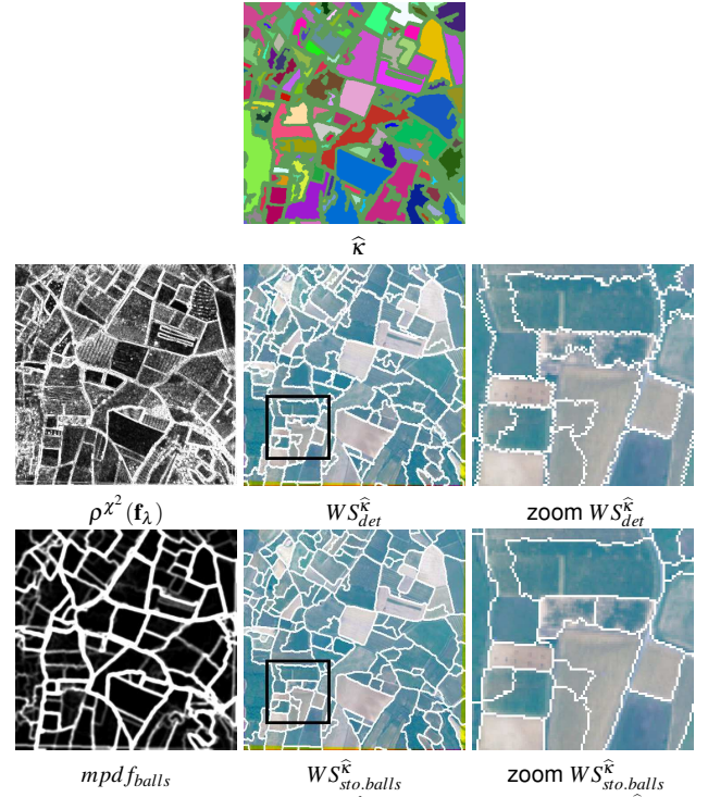
Figure 7. Filtered classification \hat{\kappa} , deterministic approach WS_{det}^{\hat{\kappa}} on Chi-squared metric based gradient \rho^{\chi^2}(\mathbf{f}_\lambda) (top) and stochastic approach WS_{sto.balls}^{\hat{\kappa}} on mpdf_{balls} (bottom) on image "Roujan". In both cases, the seeds come from \hat{\kappa} . For visualization, and for complete segmented images the contours are dilated by a se of size 3 \times 3 pixels.
