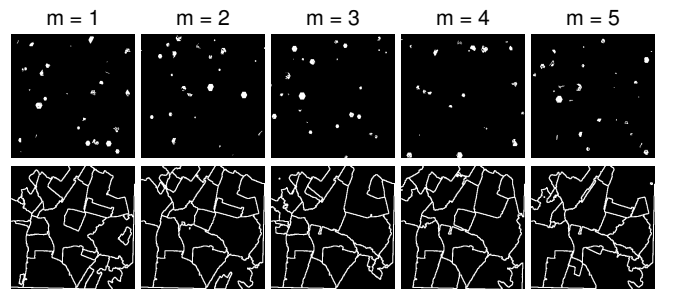
Figure 6. A few realizations of regionalized random balls markers \{mrk_m^j(x)\}_{m=1 \dots 5}^{j=1 \dots 5} (top) by the classification \hat{\kappa} and associated contours of watershed \{sgm_m^j(x)\}_{m=1 \dots 5}^{j=1 \dots 5} (bottom).
