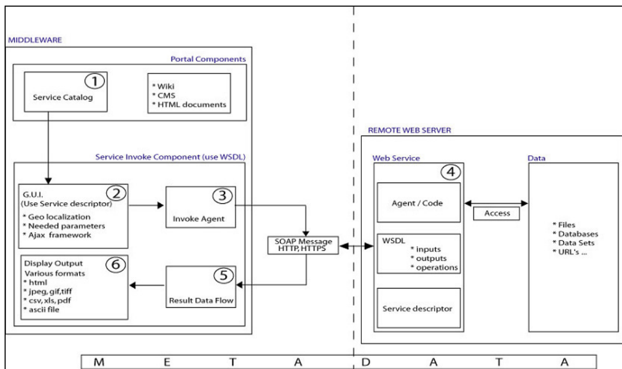
Figure 11.2: Diagram of the components and data flow in the information system
