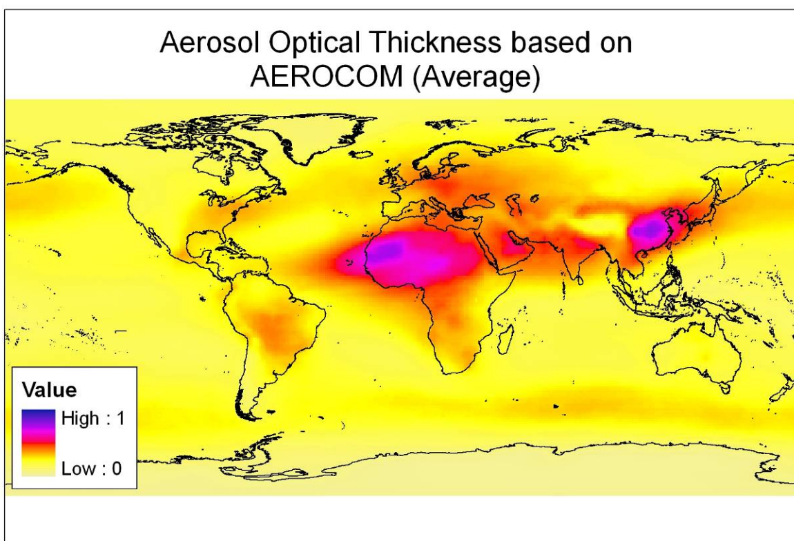
Figure 6.4: Annual average of the aerosol optical thickness for the Aeroicom data set
