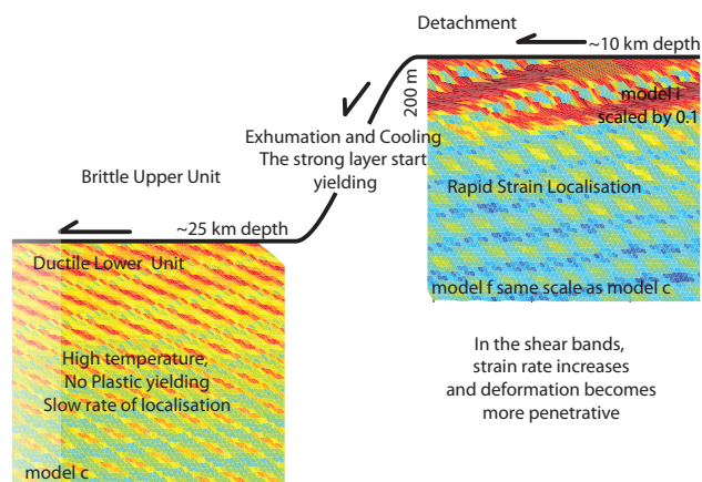
Fig. 10. Sketch model for shear localisation beneath a detachment fault. Layered rocks are initially at high temperature and large confining pressure corresponding to model c. The rapid cooling during exhumation causes the strong layers to start yielding. According to model f, this results in shear banding and rapid localisation of strain ( \gamma < 1 ). Within the shear bands, the strain rate is approximately increased by a factor of 10, corresponding to model i and resulting in more penetrative deformation and onset of mylonitisation.
