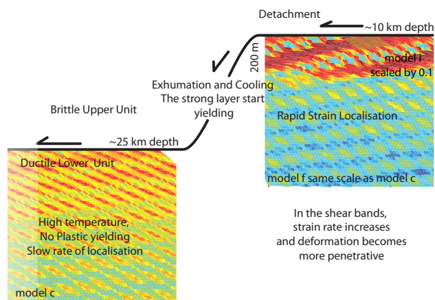
Fig. 10. Sketch model for shear localisation beneath a detachment fault. Layered rocks are initially at high temperature and large confining pressure corresponding to model c. The rapid cooling during exhumation causes the strong layers to start yielding. According to model f, this results in shear banding and rapid localisation of strain ( \gamma < 1 ). Within the shear bands, the strain rate is approximately increased by a factor of 10, corresponding to model i and resulting in more penetrative deformation and onset of mylonitisation.
