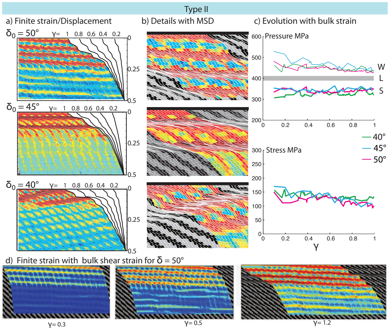
Fig. 5. Type II (a) Strain (colour scale) is maximum in shear bands rather than in weak layers. The deformed profiles for \gamma respectively equal to 0.2, 0.4, 0.6, 0.8 and 1 indicate that displacement rate decreases with time at depth. (b) In shear bands, MSD tends to be parallel to the bulk shear at large strain. (c) Pressure gap between the weak (W, thin lines) and strong (S, thick lines) as well as the deviatoric stresses decrease with time indicating, strain softening. (d) The evolution of finite strain with time for \delta_0 = 50^\circ indicates that the deeper shear bands are active from the onset of deformation.
