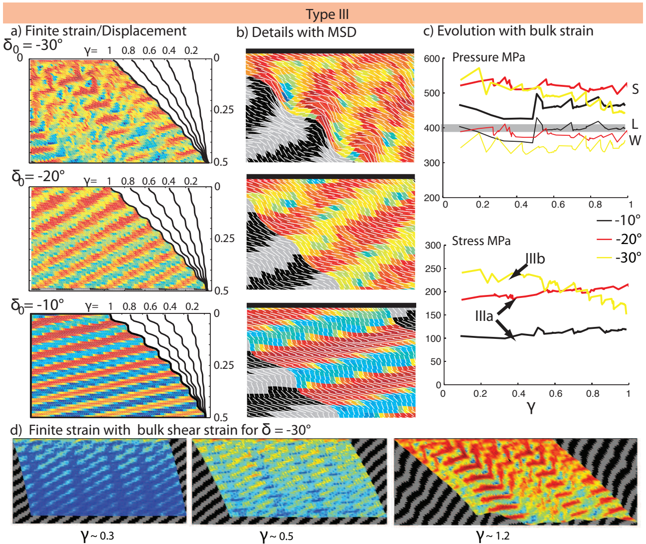
Fig. 6. Type III (a) Finite strain (colour scale) is maximum in weak layers and distributed among small-scale folds at all depths. The deformed profiles for \gamma respectively equal to 0.2, 0.4, 0.6, 0.8 and 1 indicate no localisation with time, as displacement rates are roughly constant with increasing bulk strain. (b) MSD (white lines) indicates pure thickening in strong layers. (c) Pressure in weak layers (W, thin line) is very close to lithostatic pressure (L) while pressure in strong layers (S, thick line) is higher than lithostatic. Evolution of deviatoric stresses discriminates between Type IIIa and IIIb. (d) \delta_0 = -30^\circ model is affected by kink bands that develop at the onset of strain softening.
