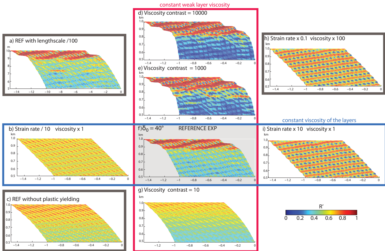
Fig. 9. Scaling of models. The reference model f is equivalent to \delta_0 = 40^\circ model. The blue box models represent the effect of varying the background strain rate. The red box models test the influence of the strength of strong layers. The grey frames denote three special runs. All changed parameters are listed in Table 1.
