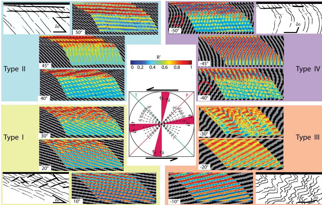
Fig. 3. Results of the parametric study at \gamma = 1 , accompanied by sketches of results. Black and grey indicate, respectively, the location of weak and strong layers; colour scale indicates strain intensity. Red circles refer to specific structures described in the text. P and T are the instantaneous shortening and stretching axis at large scale, respectively. Maximum large-scale shear directions are indicated in magenta.
