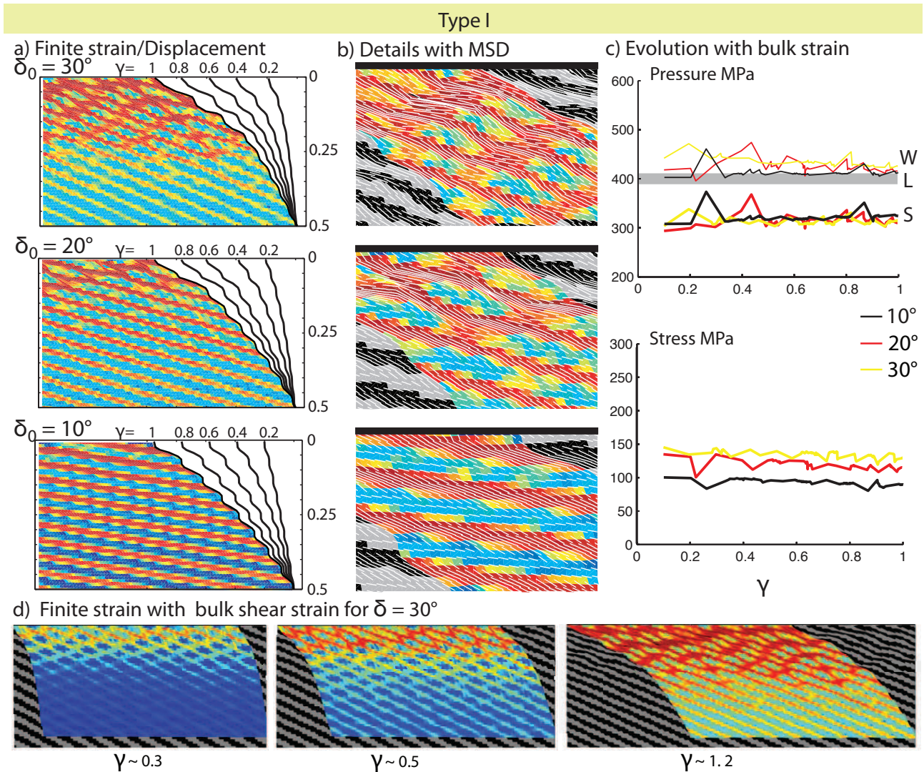
Fig. 4. Type I (a) Colour scale indicates strain intensity. Most of strain concentrates in weak layers and increases in strong layers as obliquity increases. Depth-displacement profiles (solid black lines) indicate no localisation of deformation beneath detachment with rising bulk strain. (b) MSD (white lines) indicates coaxial stretching of strong layers and shearing of weak layers. (c) Evolution of pressure and deviatoric stress for weak (W, thin lines) and strong (S, thick lines) suggest stationary stress and a pressure gap between strong and weak layers. Applied lithostatic pressure (L) is outlined by a thick grey line (d). The evolution of finite strain with time for the \delta_0 = 30^\circ model suggests that distribution of strain rate with depth is acquired at an early stage.
