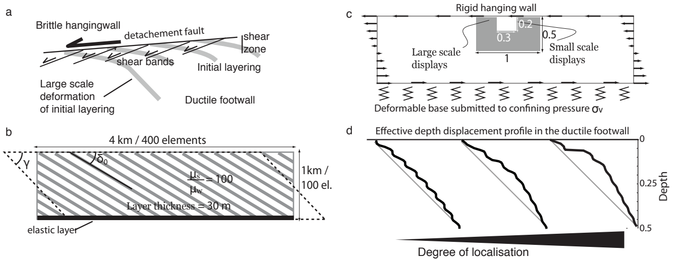
Fig. 1. (a) Sketch of a detachment fault separating a brittle upper crust (not modelled here) from the ductile footwall exhibiting a mechanical layering (grey lines). At large scale the deformation is localised close to the detachment, with a specific downward penetration. Within this zone, the initial layering is crosscut by shear bands at small scale. (b) Model set up with initial layering (grey and white layers) dipping at an angle \delta_0 . Note that an elastic layer has been placed at the base of the model. (c) Sketch of the boundary conditions with boxes representing the part of models in the subsequent figures. Confining pressure is applied on the elastic layer to avoid large pressure jumps between weak and strong layers at their base. (d) depth/displacement profiles are used to estimate the degree of strain localisation at large scale.
