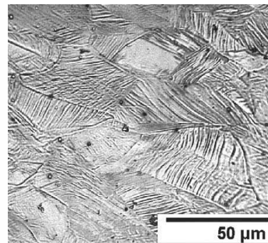
Fig3. Optical micrograph after etching to reveal grain boundaries and twins from a sample deformed at 293K [2]
