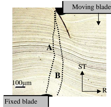
Fig8. Optical micrograph of interrupted shear specimen of Fe22Mn0.6C steel. Crack path of a Dual Phase steel (Profile A) and a 2024 aluminum alloy (Profile B) are indicated from [2].
