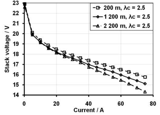
Fig. 7: Polarization curves at 200 m, 1\,200 m and 2\,200 m and at \lambda_c = 2.5 .
