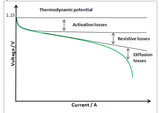
Fig. 3: Typical polarization curve of a single fuel cell.
