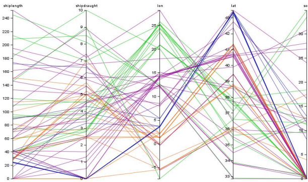
Figure 5. Parallel coordinates plot describing the profile of 70 ships (ship length, ship draught, lon, lat, speed over ground).
