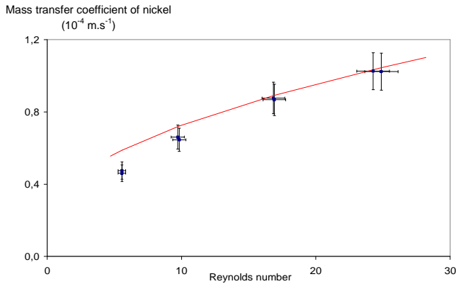
Fig. 5 Mass transfer coefficient of nickel versus Reynolds number for an inlet nickel concentration fixed at 20 mg.kg -1 ■: experimentally measured and —: calculated from Dwivedi and Upadhyay correlation [12] with D=6.6 \times 10^{-10} \text{ m}^2.\text{s}^{-1}
