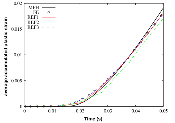
Fig. 3. Average accumulated plastic strain in the matrix after tensile deformation up to 5% for a volume fraction of the inclusions equal to 15% and at the strain rate of 1 \text{ s}^{-1} .
