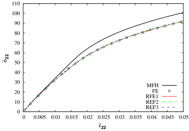
Fig. 2. Finite-element, incrementally affine homogenization, and a priori hyper reduction results of the stress–strain curves in tension test at the strain rate of 1 \text{ s}^{-1} for a volume fraction of inclusions equal to 15%.
