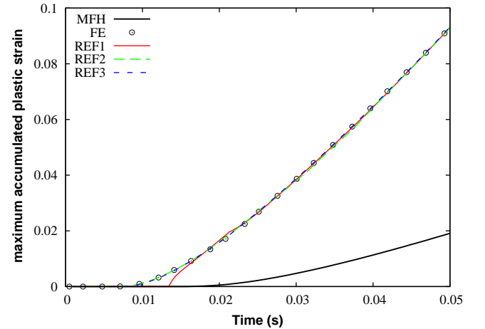
Fig. 4. Maximum accumulated plastic strain in the matrix after tensile deformation up to 5% for a volume fraction of the inclusions equal to 15% and at the strain rate of 1 \text{ s}^{-1} .
