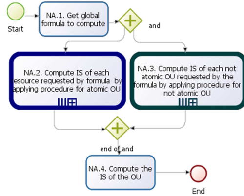
Fig. 7: Sub-process "Execute procedure for not atomic OU"
