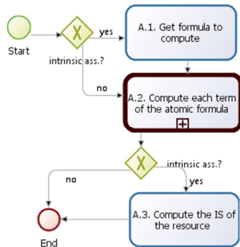
Fig. 5: Sub-process "Execute procedure for an atomic OU"
