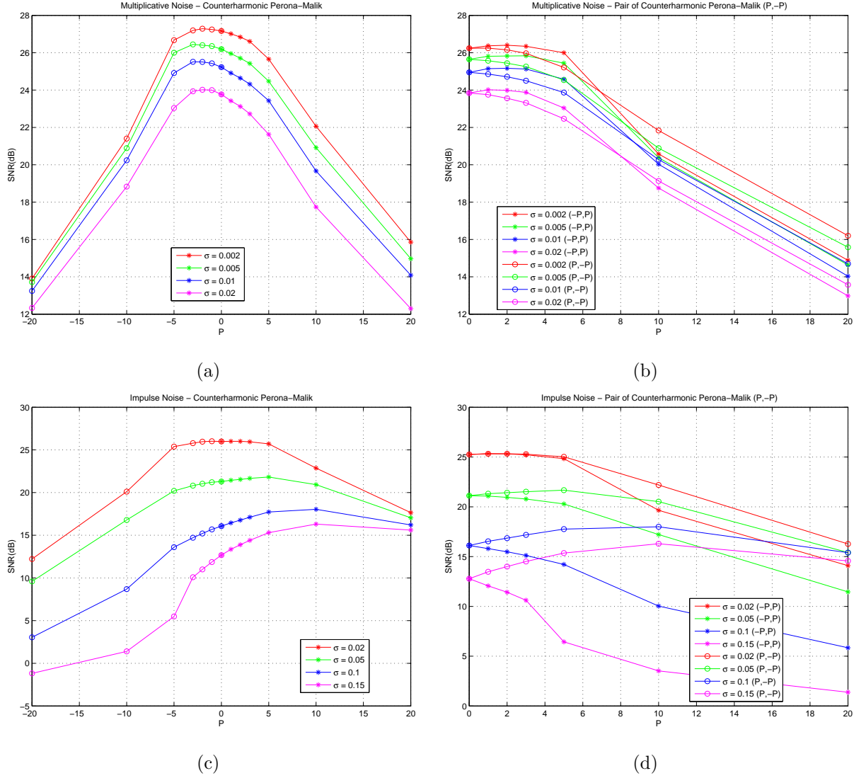
Figure 11: Denoising assessment in terms of SNR with respect to order of the generalised morphological nonlinear diffusion \xi(x, y; t; P)(f') (fixed t = 5 ): (a) pseudo-erosion \xi(x, y; t; P < 0)(f') and pseudo-dilation \xi(x, y; t; P > 0)(f') for speckle noise at four values of \sigma ; (b) pseudo-opening \xi(x, y; t; P > 0)(\xi(x, y; t; P < 0)(f')) and pseudo-closing \xi(x, y; t; P < 0)(\xi(x, y; t; P > 0)(f')) for speckle noise at four values of \sigma ; (a) pseudo-erosion \xi(x, y; t; P < 0)(f'') and pseudo-dilation \xi(x, y; t; P > 0)(f'') for asymmetric impulse noise at four values of \sigma ; (b) pseudo-opening \xi(x, y; t; P > 0)(\xi(x, y; t; P < 0)(f'')) and pseudo-closing \xi(x, y; t; P < 0)(\xi(x, y; t; P > 0)(f'')) for asymmetric impulse noise at four values of \sigma .
