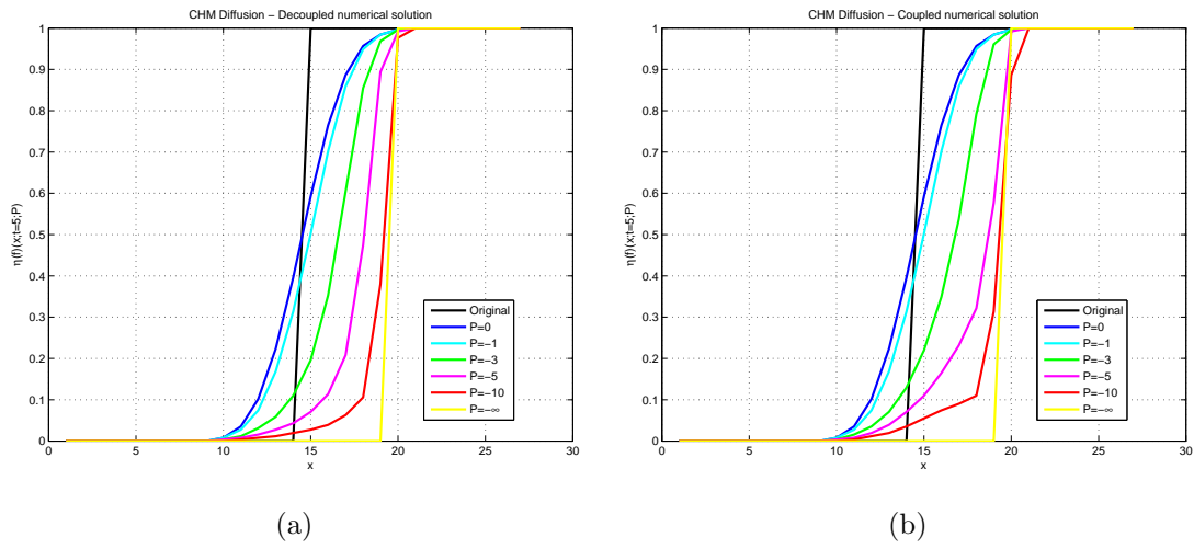
Figure 4: Comparison of CHM linear diffusion of a 1D signal using in (a) the decoupled iterative scheme \eta(f)(x, y; t; P) (a) and in (b) the coupled iterative scheme \hat{\eta}(f)(x, y; t; P) , at spatial scale t = 5 and with respect to various values of P \leq 0 .
