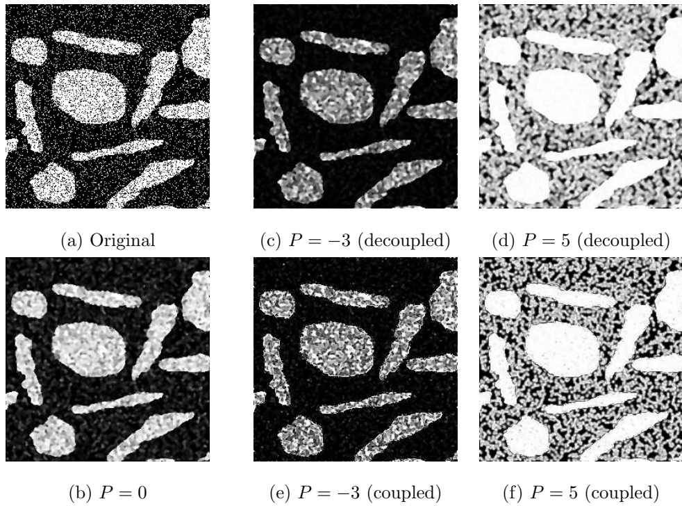
Figure 7: Comparison of decoupled and coupled generalised morphological Perona and Malik diffusion \xi(x, y; t; P) at scale t = 5 (regularization parameter \sigma = 0.5 ): (a) original image, (b) standard nonlinear diffusion, (c)/(d) pseudo-dilation/erosion by counter-harmonic nonlinear diffusion using decoupled schema, (e)/(f) pseudo-dilation/erosion by counter-harmonic nonlinear diffusion using coupled schema.
