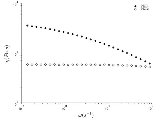
Figure 3: Viscosity as a function of frequency for both polyesters at 260^\circ\text{C} (deduced from complex modulus measurement on a cone and plate RMS 800 Rheometer)
