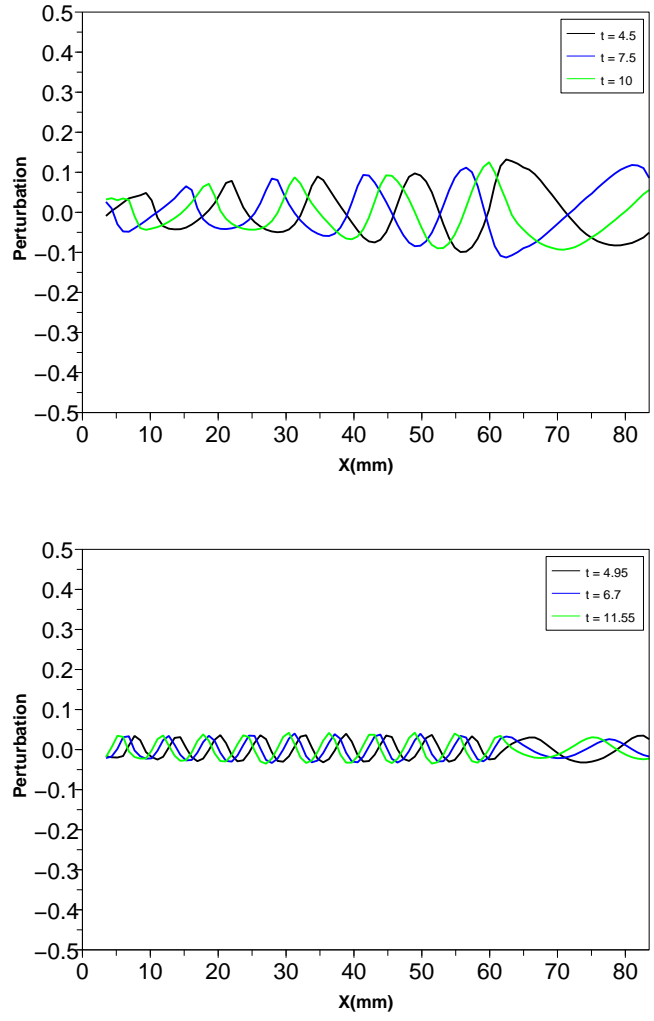
Figure 15: Case N o 4 and 30° angle in the convergent geometry. Perturbation along flow motion for various time steps; a) forcing frequency 0.5 Hz, b) forcing frequency 1 Hz
