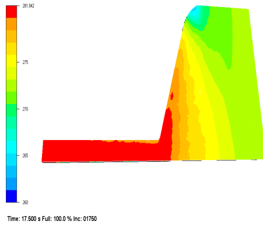
Figure 6: Mean temperature distribution in the die: the inlet temperature is 281^{\circ}C , die temperature is 260^{\circ}C ; same flow rate as in figure 5
