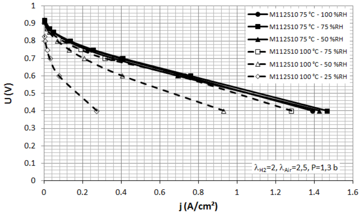
Figure 10. Polarization curves obtained for M112S10, at 75 °C (solid lines) and 100 °C (dashed lines), between 25 and 100% relative humidity.
