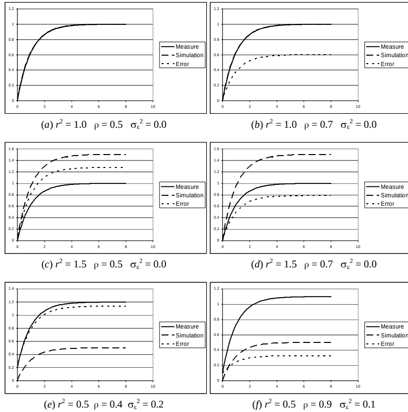
Figure 2. Some configurations of variograms, depending on the ratio r , the correlation \rho , and the measurement error variance \sigma_e^2 .
