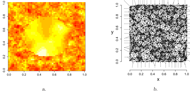
Fig. 1 Example dataset: full realization a. and Delaunay triangulation corresponding to the sampling performed b.
