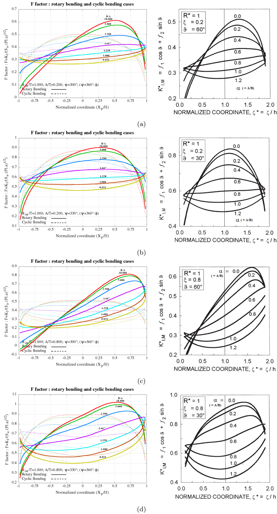
Figure 6: Comparisons with the results of Carpinteri [5]: (a) R_{int}/T = 1, A/T = 0.2, \psi = 60^\circ and different values of B/A , (b) R_{int}/T = 1, A/T = 0.2, \psi = 30^\circ and different values of B/A , (c) R_{int}/T = 1, A/T = 0.8, \psi = 60^\circ and different values of B/A , (d) R_{int}/T = 1, A/T = 0.8, \psi = 30^\circ and different values of B/A .
