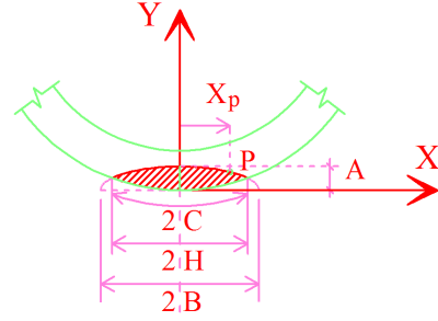
(b) Crack geometry and parameters
