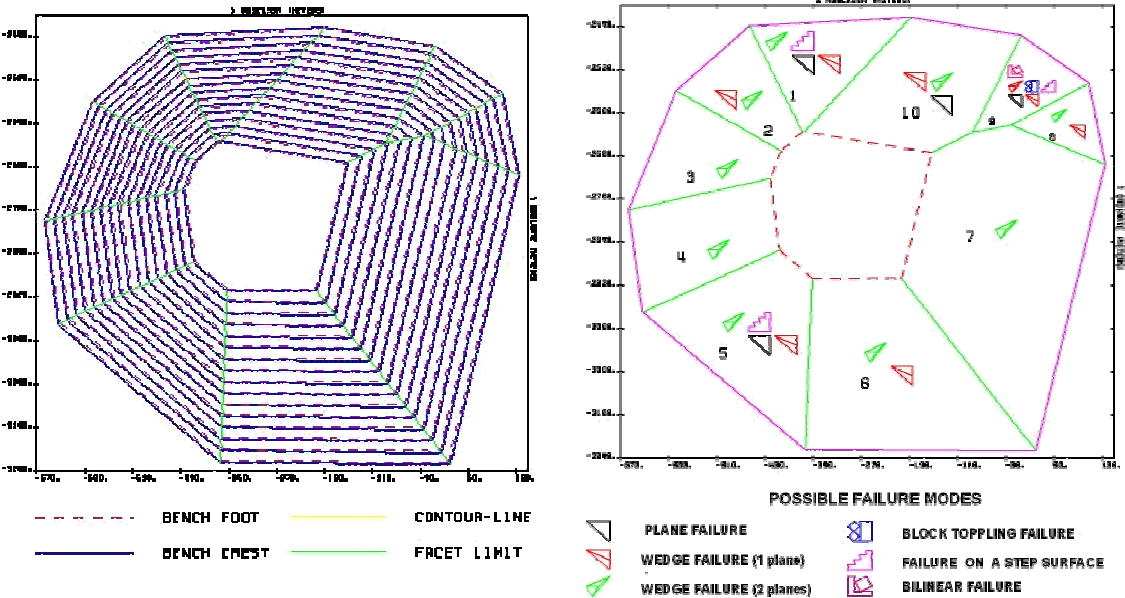
Figure 2: Geometrical pit model (left) and detection of the failure risks (right) using the DEGRES software
