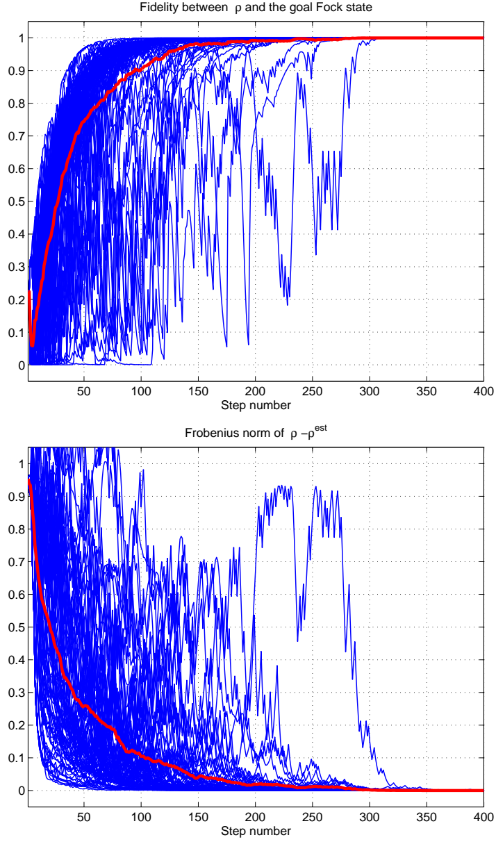
Figure 5: (First plot) \text{Tr}(\rho_k \bar{\rho}) = \langle 3|\rho_k|3\rangle versus k \in \{0, \dots, 400\} for 100 realizations of the closed-loop Markov process (2) with feedback (20) based on the quantum filter (19) starting from the same state \chi_0^{\text{est}} = (\frac{1}{n^{\text{max}+1} \mathbb{I}_{(n^{\text{max}+1)} \times (n^{\text{max}+1)}}, 0, \dots, 0) with 5-step delay ( d = 5 ). The initial state of the physical system \rho_0 is given by \mathbb{D}_{\sqrt{3}}(|0\rangle\langle 0|) . The ensemble average over these realizations corresponds to the thick red curve; (Second plot) The Frobenius distance between the estimator \rho^{\text{est}} and \rho ( \sqrt{\text{Tr}((\rho - \rho^{\text{est}})^2)} ) for 100 realizations. The ensemble average over these realizations corresponds to the thick red curve.
