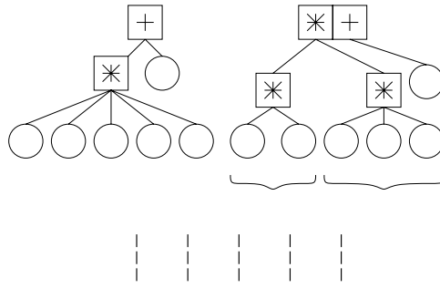
Figure 10: Heuristics example.
