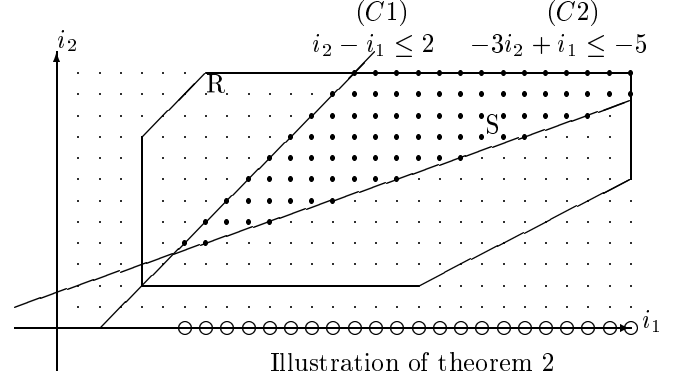
Illustration of theorem 2
