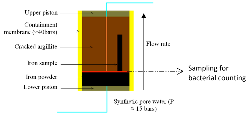
Fig. 1. Schematic view of the experimental cell
