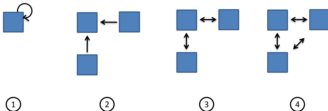
Figure 2 Four strategies of modelling global production chains.
