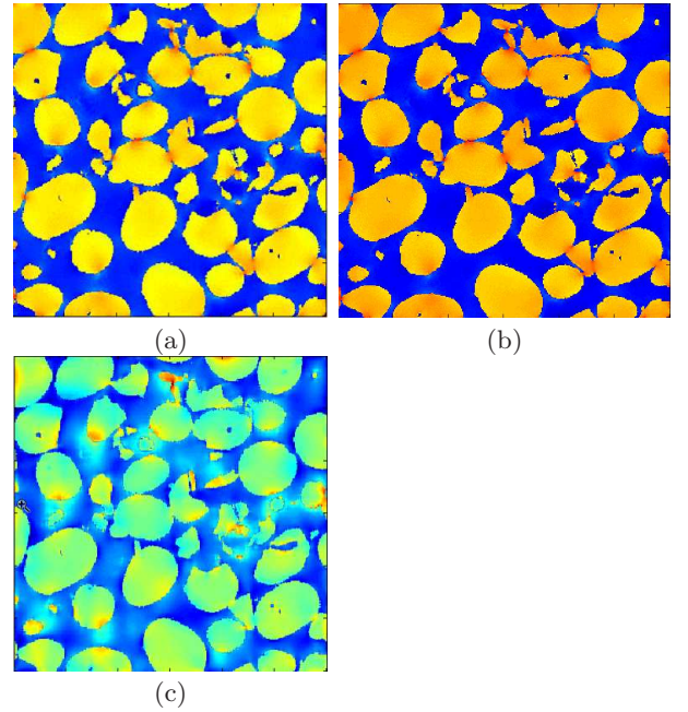
FIG. 13. Maps of the mean and shear strain components \varepsilon_m (a, b) and \varepsilon_{12} (c), with applied hydrostatic strain loading \langle \varepsilon_{ij}(\mathbf{x}) \rangle = \varepsilon^{(0)} \delta_{ij} and shear along 1,2 i.e. \langle \varepsilon_{ij}(\mathbf{x}) \rangle = \varepsilon^{(0)} (\delta_{i1} \delta_{j2} + \delta_{i2} \delta_{j1}) , respectively. In maps (a) and (b), the Poisson ratios in the matrix and inclusions is \nu = 0 and \nu = 0.2 resp., whereas \nu = 0 in (c). The local fields maxima are shown in red, with smallest values in blue.
