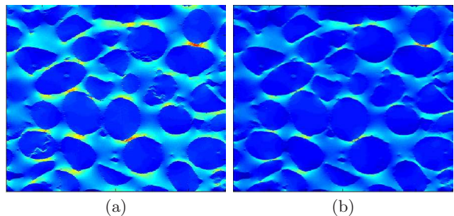
FIG. 8. Maps of the temperature gradient component \partial_i T(\mathbf{x}) along a 2D section x_3 = cste with x_1 and x_2 directed downward and rightward, respectively, for the connected (a) and unconnected (b) microstructures. The component \partial_i T(\mathbf{x}) is parallel to the applied field, i.e. \langle \partial_i T(\mathbf{x}) \rangle = \Delta T^{(0)} \delta_{i1} .
