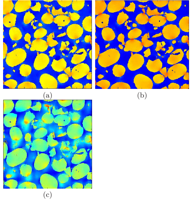
FIG. 13. Maps of the mean and shear strain components \epsilon_m (a, b) and \epsilon_{12} (c), with applied hydrostatic strain loading \langle \epsilon_{ij}(\mathbf{x}) \rangle = \epsilon^{(0)} \delta_{ij} and shear along 1, 2 i.e. \langle \epsilon_{ij}(\mathbf{x}) \rangle = \epsilon^{(0)} (\delta_{i1} \delta_{j2} + \delta_{i2} \delta_{j1}) , respectively. In maps (a) and (b), the Poisson ratios in the matrix and inclusions is \nu = 0 and \nu = 0.2 resp., whereas \nu = 0 in (c). The local fields maxima are shown in red, with smallest values in blue.
