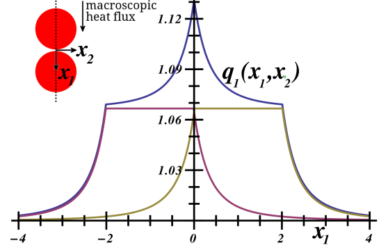
FIG. 14. Heat flux component q_1(x_1, x_2) (blue curve) along the line x_2 \equiv 0 passing through the centers of two closely-packed spheres (dotted line, top-right) as a function of the coordinate x_1 . A macroscopic heat flux is applied far from the spheres so that \langle q_i(x_1, x_2) \rangle = \delta_{i1} and the contrast of conductivity between the spheres and the matrix is small: \lambda^{inc}/\lambda^{(m)} = 1.1 . Points (x_1, x_2) = (-1.005, 0) , (1.005, 0) and (0, 0) refer to the two sphere centers and to the center between the two spheres, respectively, i.e. the spheres radius is 1 and the distance between the spheres is 0.01. Shown in red and brown are the contributions of each sphere, equal to the heat flux component q_1 if it was alone in the matrix.
