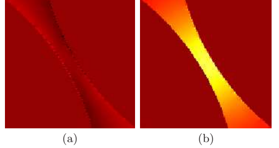
FIG. 17. Transverse (a) and normal (b) components of the heat flux vector occurring in a gap located in-between two randomly oriented, closely-packed infinitely-conducting inclusions. The transverse component in (a), orthogonal to the inclusion frontiers in the gap, is close to 0 (brown) whereas the normal component in (b), parallel to the inclusion frontiers, is close to a field that, in the matrix, depends solely on the transverse coordinate (in yellow-red colors).
