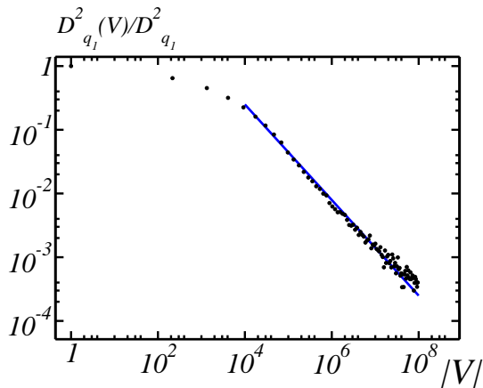
FIG. 5. Variance D_{q_1}^2(V) of the heat flux field q_1(\mathbf{x}) over a subvolume V , as a function of the volume size |V| in log-log scale (black points). The macroscopic gradient \langle \partial_i T(\mathbf{x}) \rangle = \Delta T^{(0)} \delta_{i1} is enforced over the whole volume \Omega . The variance D_{q_1}^2(V) is normalized by the point variance D_{q_1}^2 ; the ratio behaves as \simeq A_3/|V| (blue curve) when |V| is much larger than the integral range A_3 .
