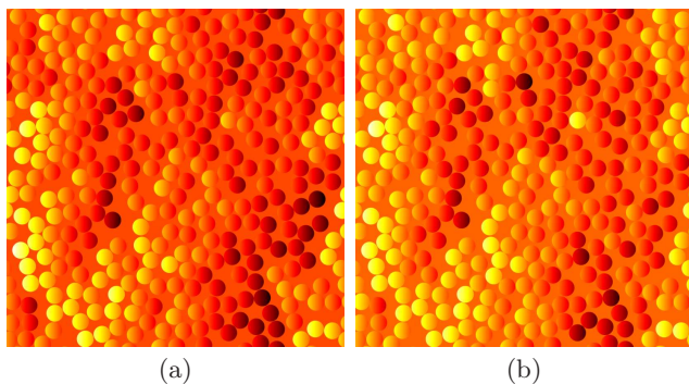
FIG. 19. Periodic part of the temperature field T(\mathbf{x}) - \Delta T_i^{(0)} x_i in the hard-core Boolean model with infinitely-conducting cylinders. Comparison between FFT exact results (a) and the “network model” (b), with highest and lowest values shown in white and red, respectively.
