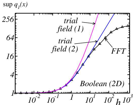
FIG. 15. Maximum of component 1 of the heat flux q_1(\mathbf{x}) in the matrix and inclusions as a function of the contrast h in log-log scale, for a Boolean set of cylinders of concentration 30%: comparison between FFT results and estimates given by the trial fields \mathbf{E}^* from Eq. (6.7) with the choice t = h (trial field 1, magenta) or t as in Eq. (6.8) (trial field 2, blue). A macroscopic temperature gradient is applied in direction 1 so that \langle \partial_i T(\mathbf{x}) \rangle = \partial_{i1} \Delta T^{(0)} with \Delta T^{(0)} = 1 . When h is small, the maximum of the heat flux q_1(\mathbf{x}) behaves as \approx 1 + 1.4h , close to the trial fields prediction, and tends to the finite value \sim 181 when h = +\infty , whereas the trial field estimates predict an infinite value.
