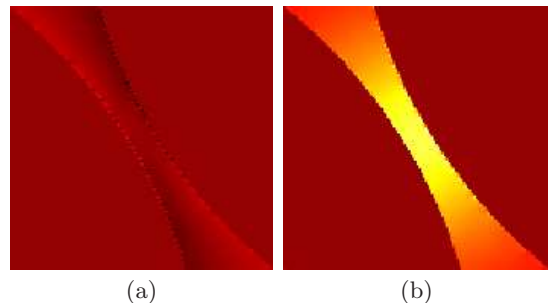
FIG. 17. Transverse (a) and normal (b) components of the heat flux vector occurring in a gap located in-between two randomly oriented, closely-packed infinitely-conducting inclusions. The transverse component in (a), orthogonal to the inclusion frontiers in the gap, is close to 0 (brown) whereas the normal component in (b), parallel to the inclusion frontiers, is close to a field that, in the matrix, depends solely on the transverse coordinate (in yellow-red colors).
