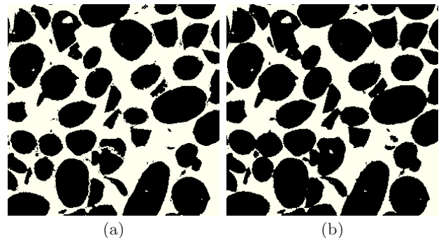
FIG. 4. Corresponding detail of 2D sections of the “connected” (a) and “unconnected” (b) microstructures.
