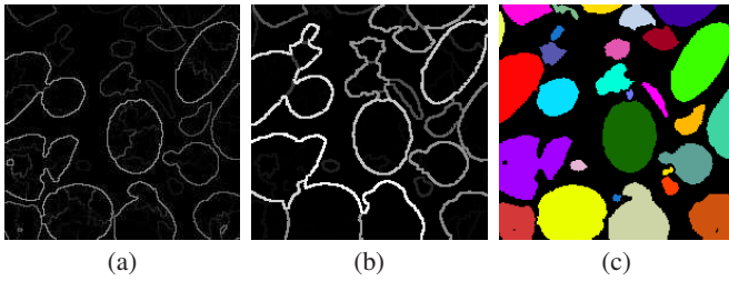
FIG. 3. Probability density function (PDF) of contours estimated with 50 realizations of a Poisson point process in 3D (a), computed with a graph-based approach (b) and graph-based stochastic watershed segmentation (c).
