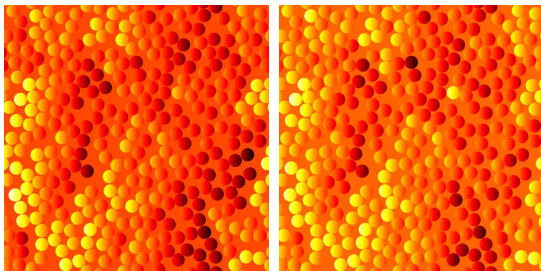
FIG. 19. Periodic part of the temperature field T(\mathbf{x}) - \Delta T_i^{(0)} x_i in the hard-core Boolean model with infinitely-conducting cylinders. Comparison between FFT exact results and the “network model”, with highest and lowest values shown in white and red, respectively.
