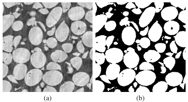
FIG. 2. Detail of a 2D section of a X-ray microtomography image of the granular material (a), and its corresponding segmentation by maximization of the interclass variance (b).
