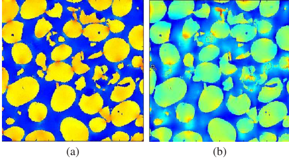
FIG. 13. Maps of the mean and shear strain components \varepsilon_m (a) and \varepsilon_{12} (b), with applied hydrostatic strain loading \langle \varepsilon_{ij}(\mathbf{x}) \rangle = \varepsilon^{(0)} \delta_{ij} and shear along 1, 2, \langle \varepsilon_{ij}(\mathbf{x}) \rangle = \varepsilon^{(0)} (\delta_{i1} \delta_{j2} + \delta_{i2} \delta_{j1}) , respectively. The local fields maxima are shown in red, whereas smallest values are in blue.
