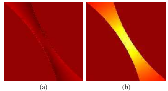
FIG. 17. Transverse (a) and normal (b) components of the heat flux vector occurring in a gap located inbetween two randomly oriented, closely-packed infinitely-conducting inclusions. The transverse component in (a), orthogonal to the inclusion frontiers in the gap, is close to 0 (brown) whereas the normal component in (b), parallel to the inclusion frontiers, is close to a field that, in the matrix, depends solely on the transverse coordinate (in yellow-red colors).
