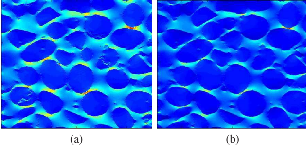
FIG. 8. Maps of the temperature gradient component \partial_1 T(\mathbf{x}) along a 2D section x_3 = cste with x_1 and x_2 directed downward and rightward, respectively, for the connected (a) and unconnected (b) microstructures. The component \partial_1 T(\mathbf{x}) is parallel to the applied field, i.e. \langle \partial_i T(\mathbf{x}) \rangle = \Delta T^{(0)} \delta_{i1} .
