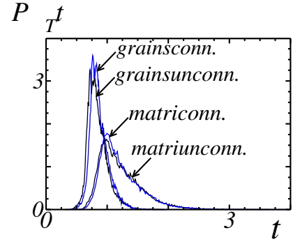
FIG. 11. Probability distribution P_{\partial_1 T}(t) of the values of the temperature gradient component \partial_1 T(\mathbf{x}) in the grains and in the matrix (blue and black, respectively), for the connected and unconnected microstructures (labelled conn. and unconn., respectively). The component \partial_1 T(\mathbf{x}) is parallel to the applied field, i.e. \langle \partial_i T(\mathbf{x}) \rangle = \Delta T^{(0)} \delta_{i1} with \Delta T^{(0)} = 1
