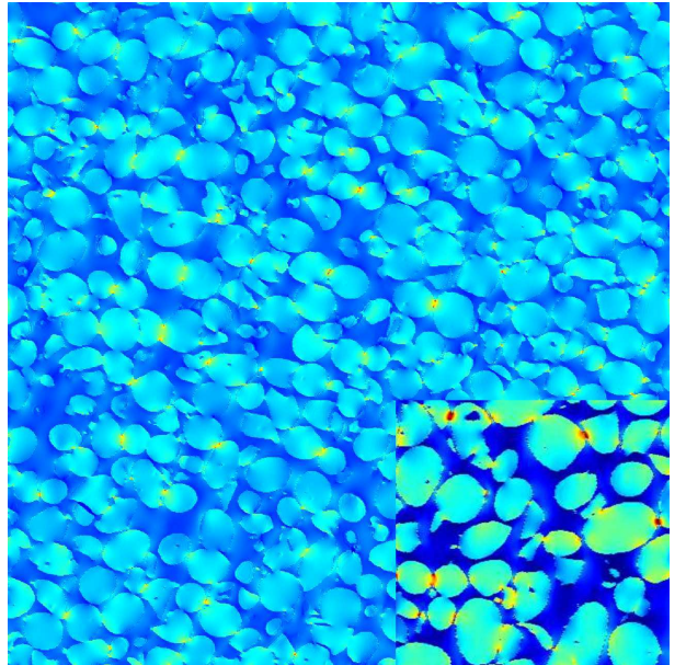
FIG. 6. 2D section of the heat flux component q_1 + q_2 occurring in the granular microstructure with blue and red zones corresponding to the local minima and maxima, respectively (bottom right: enlarged detail). A macroscopic temperature gradient is applied along (1, 1, 0) , i.e. \langle \partial_i T(\mathbf{x}) \rangle = \Delta T^{(0)} (\delta_{i1} + \delta_{i2}) . The minimum and maximum values are -2.1 and 7.4 respectively, when \Delta T^{(0)} = 1 .
