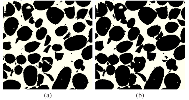
FIG. 4. Corresponding details of 2D sections of the ‘‘connected’’ (a) and ‘‘unconnected’’ (b) microstructures.
