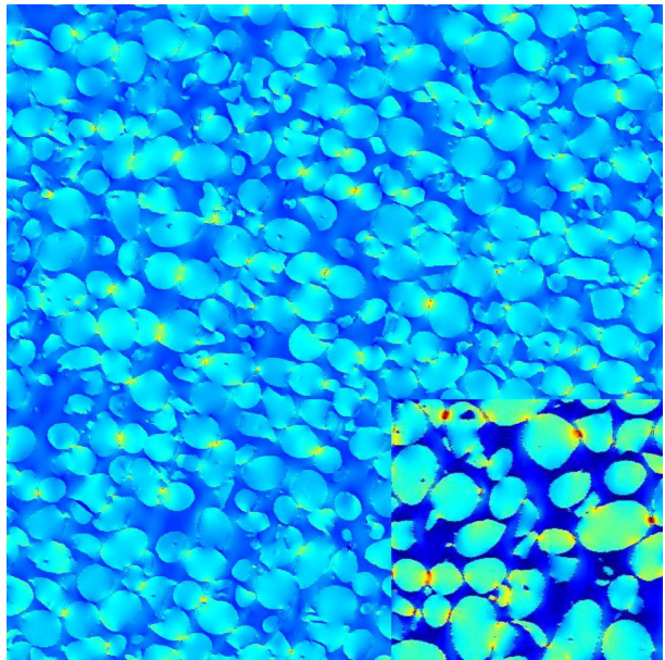
FIG. 6. 2D section of the heat flux component q_1 + q_2 occurring in the granular microstructure with blue and red zones corresponding to the local minima and maxima, respectively (bottom right: enlarged detail). A macroscopic temperature gradient is applied along (1, 1, 0) , i.e. \langle \partial_i T(\mathbf{x}) \rangle = \Delta T^{(0)} (\delta_{i1} + \delta_{i2}) . The minimum and maximum values are -2.1 and 7.4 respectively, when \Delta T^{(0)} = 1 .
