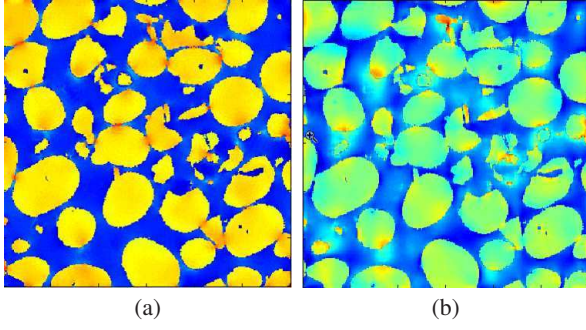
FIG. 13. Maps of the mean and shear strain components \varepsilon_m (a) and \varepsilon_{12} (b), with applied hydrostatic strain loading \langle \varepsilon_{ij}(\mathbf{x}) \rangle = \varepsilon^{(0)} \delta_{ij} and shear along 1, 2, \langle \varepsilon_{ij}(\mathbf{x}) \rangle = \varepsilon^{(0)} (\delta_{i1} \delta_{j2} + \delta_{i2} \delta_{j1}) , respectively. The local fields maxima are shown in red, whereas smallest values are in blue.
