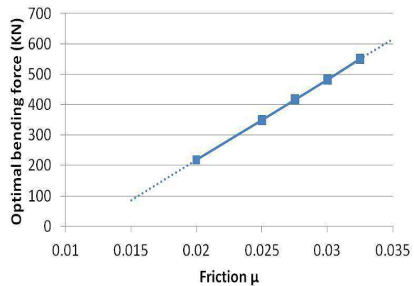
Fig. 6 The relationship between friction and optimal bending force
