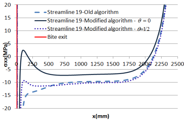
Figure 6. Stress along streamline 19 (edge) after bite exit, before and after the change of integration scheme. Stress scale is zoomed around \sigma_c = -10MPa .
