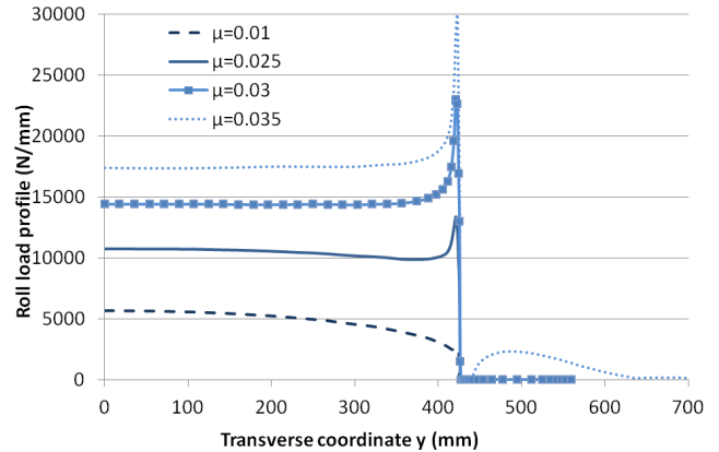
Figure 12. Roll load transverse distribution F(y) .
