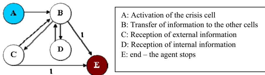
Figure 1: Behavior of the Pilot/Co-pilot Agent
