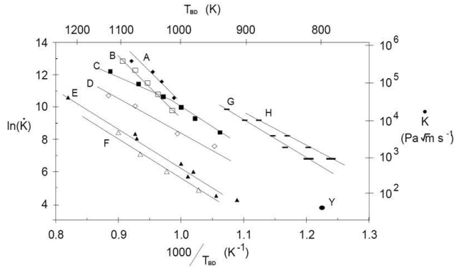
Fig. 2 Brittle-ductile transition temperature in silicon. Data from: ABC [58], D [57], EF [62], GH [59]. Doping levels: ABCH n-type, and DEFGH intrinsic
